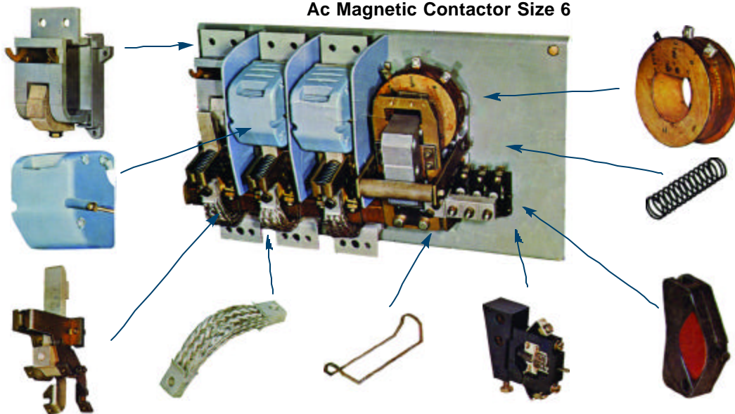
Ac Magnetic Contactor Size 6
